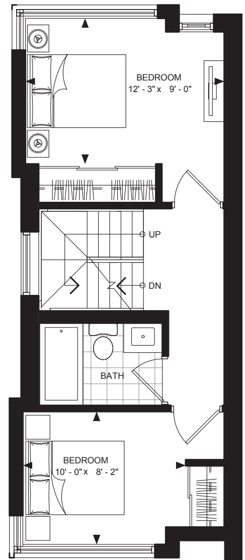
SECOND FLOOR
