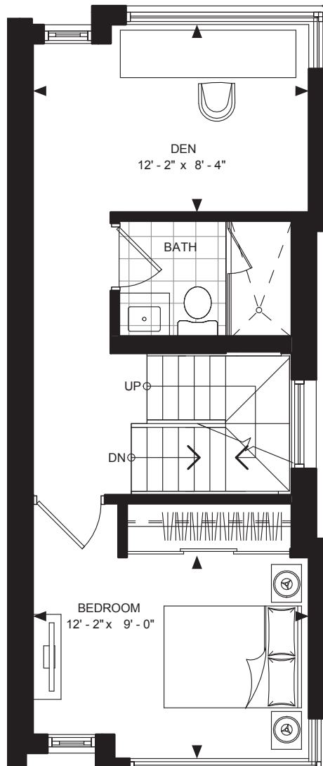
THIRD FLOOR
