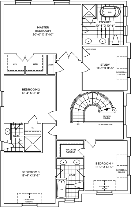
SECOND FLOOR ELEVATION B, C
