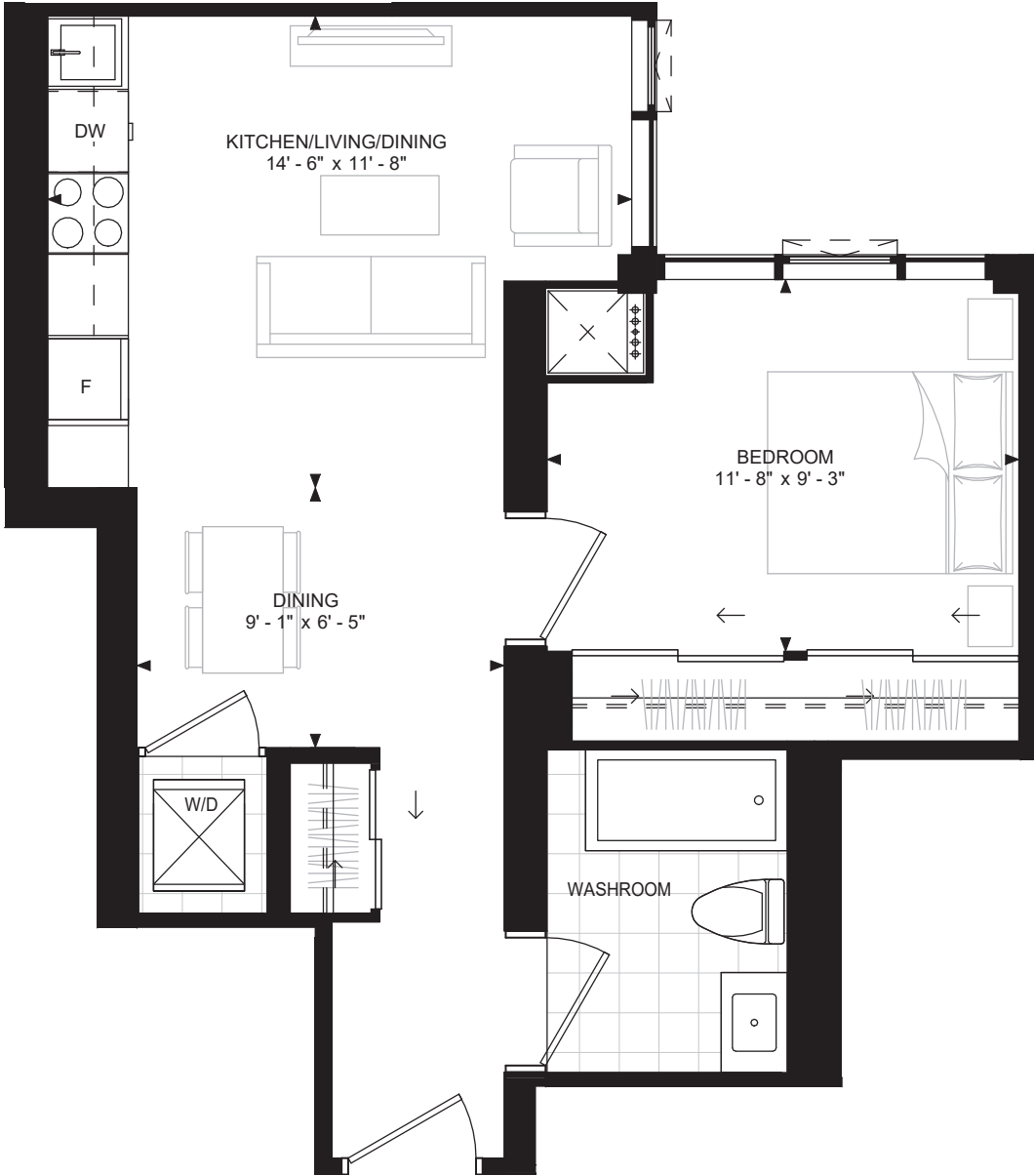
FLOOR 11 UNIT 1126 SLAB TO SLAB HEIGHT 9'6"
